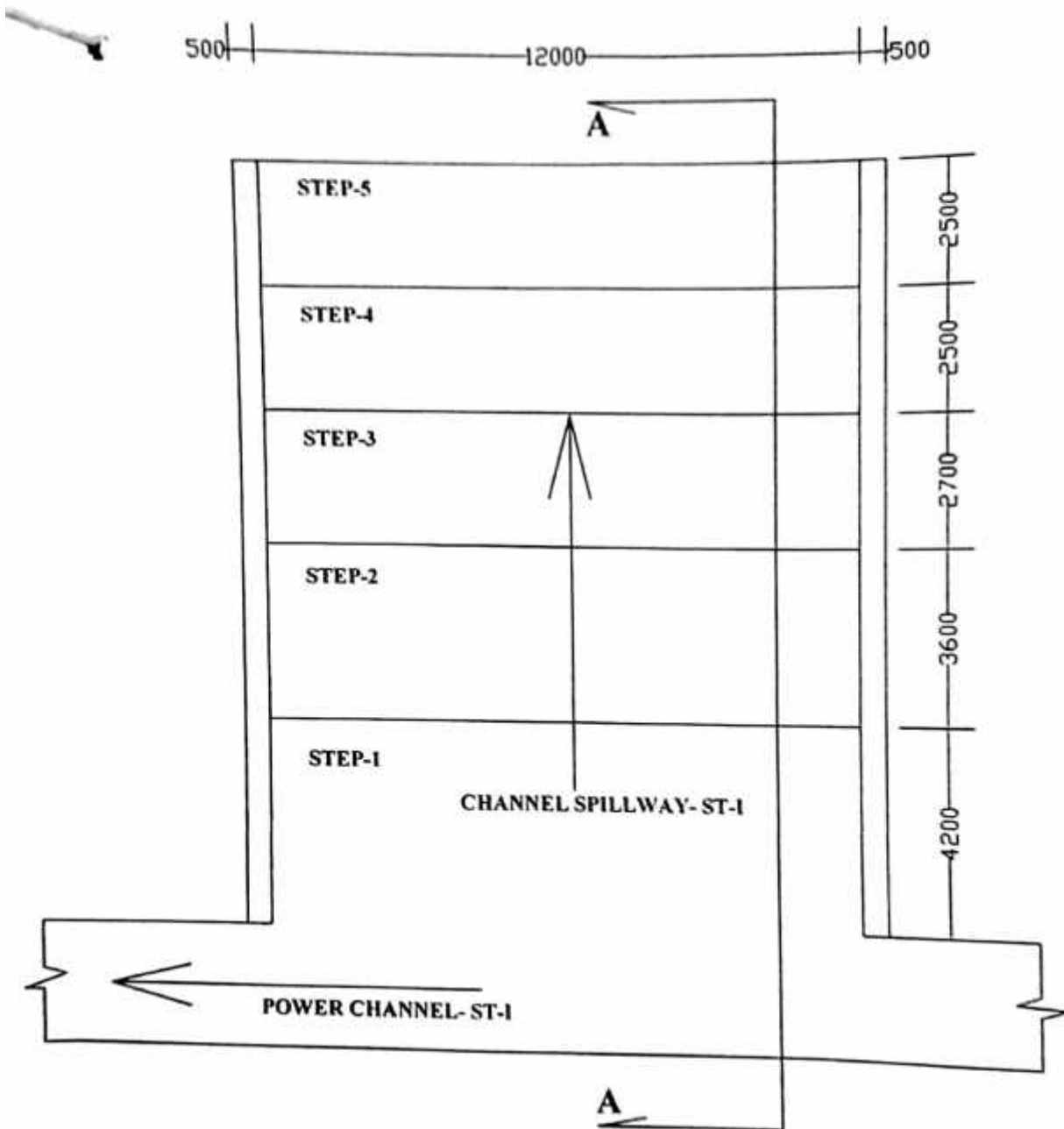
PLAN OF CHANNEL SPILLWAY, MSHEP, ST-1
